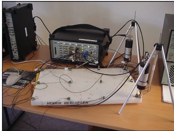
Fig. 17 Plate structure which exhibits two modes (torsional and bending) at (almost) the same frequency.
