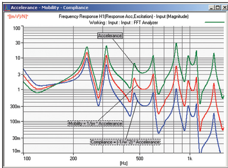
Fig. 1 displays an example of the three mobility functions (accelerance, mobility and compliance) from a structure. An accelerometer is used for the response measurement. The mobility and the compliance functions are calculated from the accelerance, by dividing by (j\omega) and -(\omega)^2 respectively. The x- and y-axes are logarithmic so that the difference between the three functions appears in the slope. The y-axis values for the three functions
