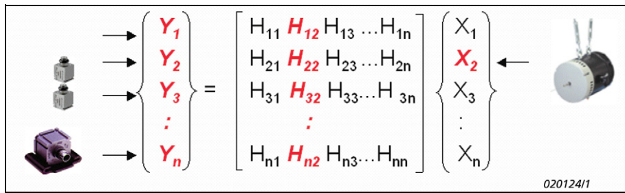
Fig. 8 Fixed shaker test with a single excitation (reference) DOF. The response transducer(s) must be moved around unless there are as many transducers available as there are response DOFs
