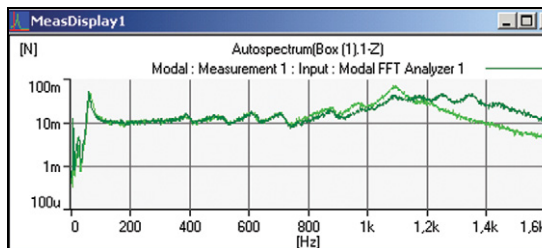
Fig. 20 Autospectra of the two force signals
